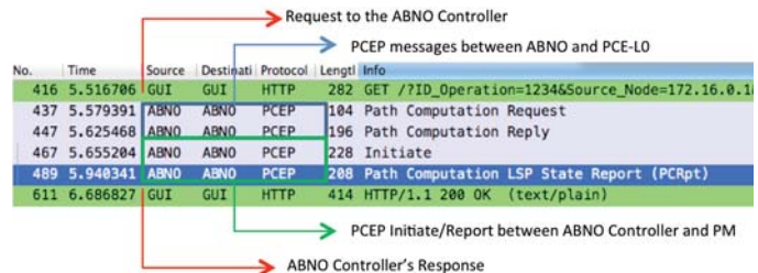
Fig. 3. Message flow in optical service provisioning use case.
